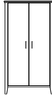
Double Wardrobe No.IS-DW41 Overall 41W x 27 3/4D x 76H Interior 38 1/2W x 25 1/4D x 71H
