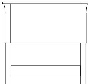
Twin Headboard - Free Standing No. IN-HB39 40 1/2W x 1 1/2D x 40H
