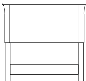
Twin Headboard - Free Standing No. FO-HB39 40 1/2W x 1 1/2D x 40H
