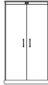
Double Wardrobe No.BH-DW41 Overall 41W x 27 3/4D x 76H Interior 38 1/2W x 25 1/4D x 71H
